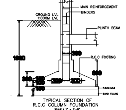
TYPICAL SECTION OF R.C.C COLUMN FOUNDATION SCALE 1"=2'-0"
