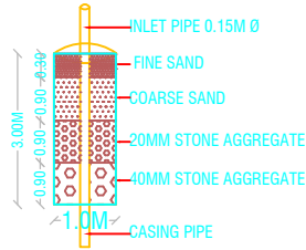
DETAILS OF RAIN WATER HARVESTING STRUCTURES
