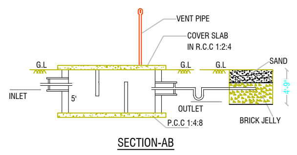
SEPTIC TANK & DISPERSION TRENCH DETAILS SCALE- 1:100
