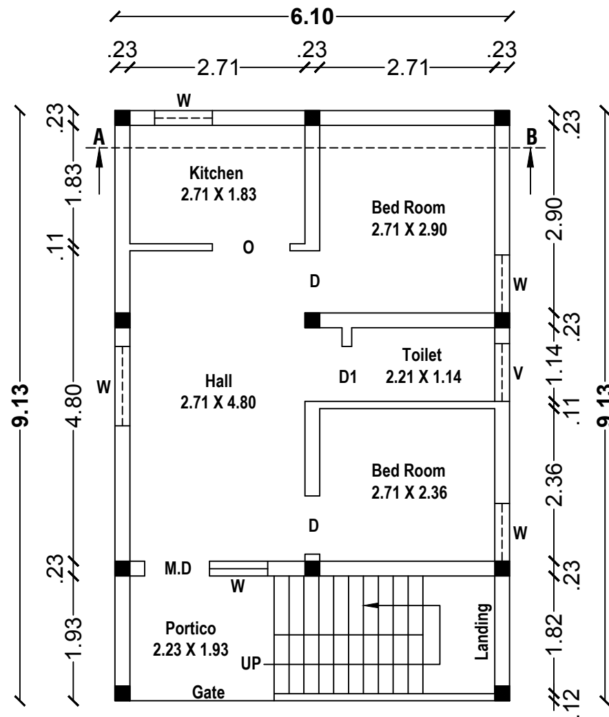
Groun Floor Plan
