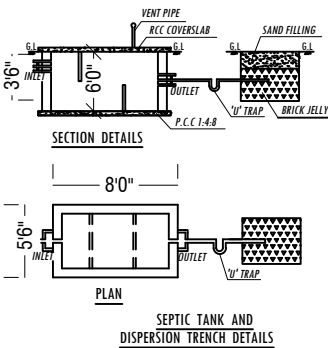
SEPTIC TANK AND DISPERSION TRENCH DETAILS
