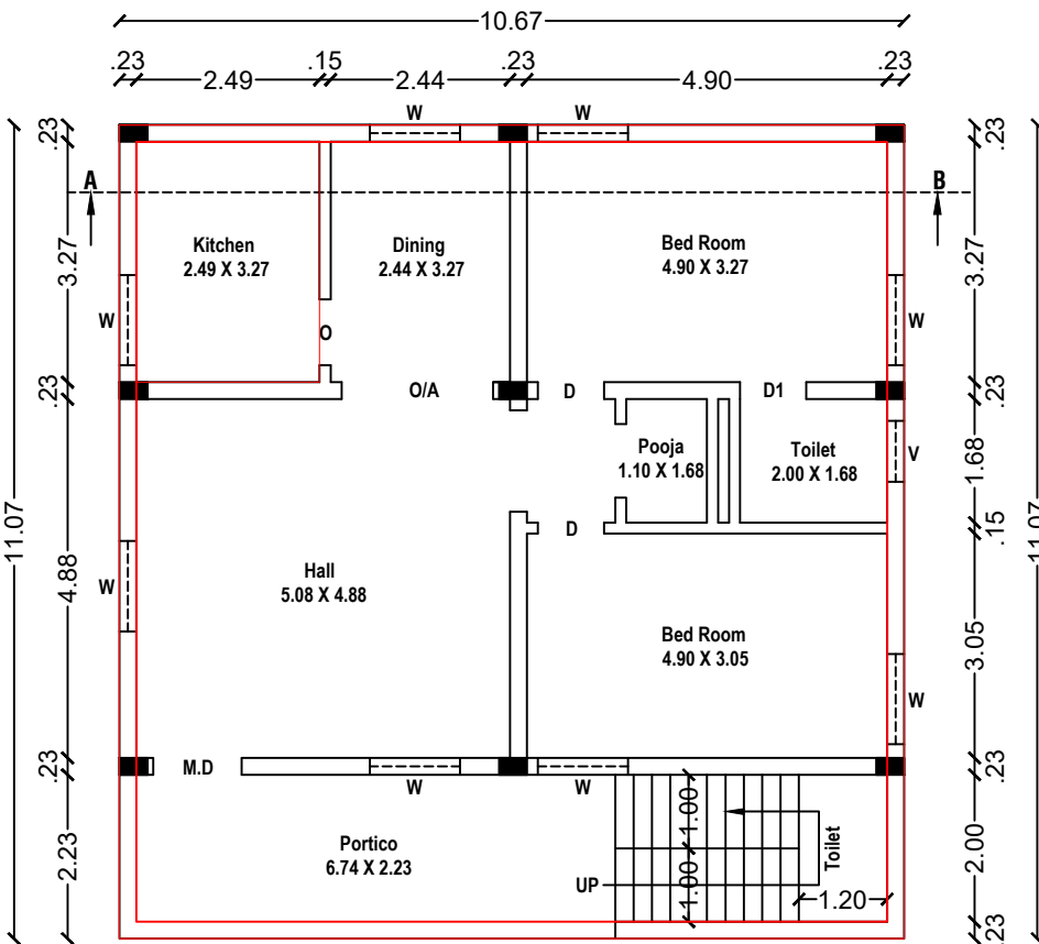
Groun Floor Plan
