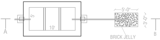
SEPTIC TANK & DISPERSION TRENCH DETAILS
