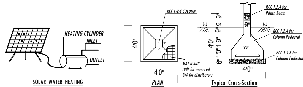
FOOTING DETAILS
