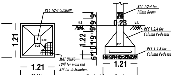
FOOTING DETAILS
