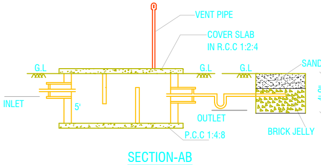
SECTION-AB
