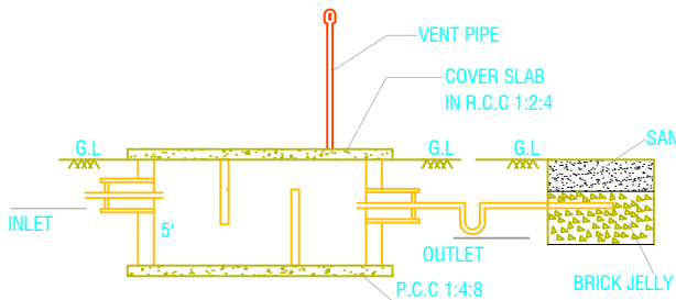
SECTION-AB
