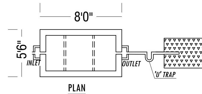
SEPTIC TANK AND DISPERSION TRENCH DETAILS
