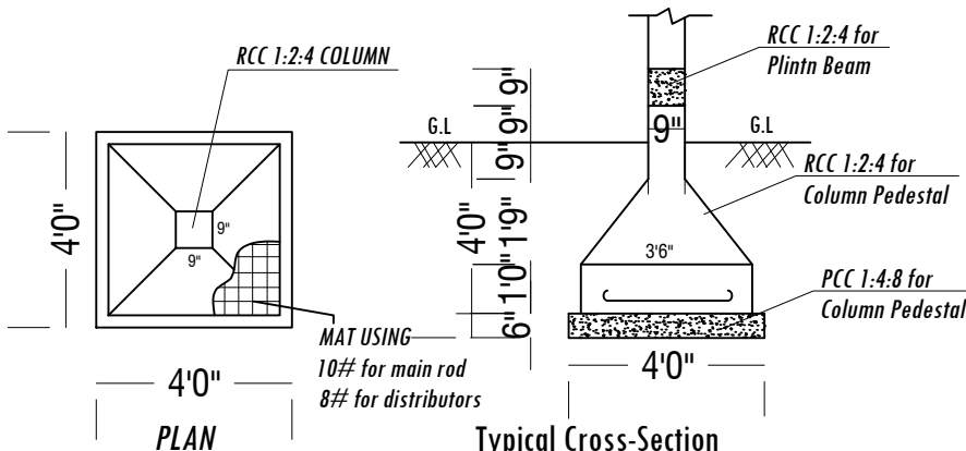
FOOTING DETAILS
