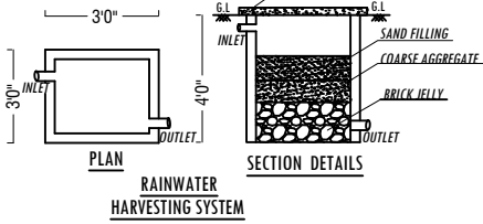
RAINWATER HARVESTING SYSTEM
