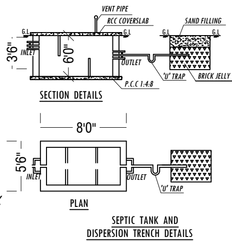
SEPTIC TANK AND DISPERSION TRENCH DETAILS
