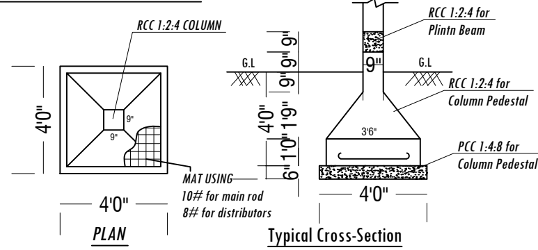
Typical Cross-Section
