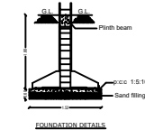
FOUNDATION DETAILS
