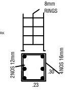
COLUMN DETAILS
