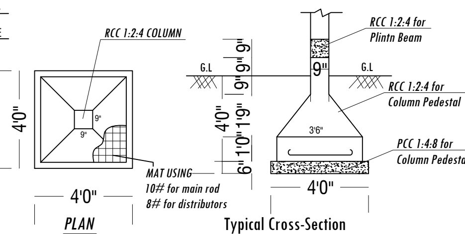
FOOTING DETAILS
