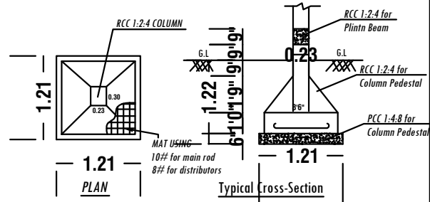
FOOTING DETAILS
