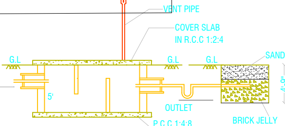
SECTION-AB
