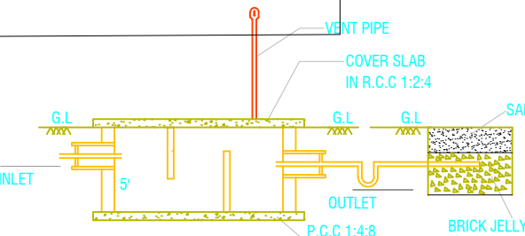
SECTION-AB
