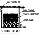
RAINWATER HARVESTING SYSTEM
