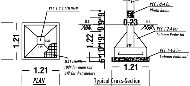
FOOTING DETAILS
