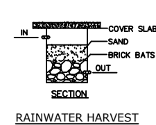
RAINWATER HARVEST
