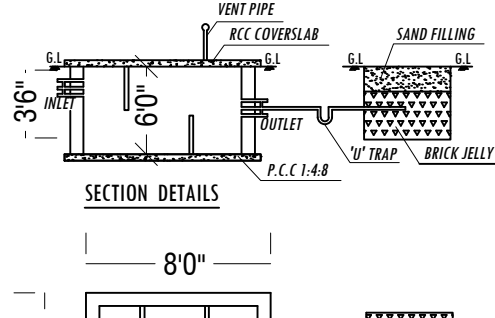
SEPTIC TANK AND DISPERSION TRENCH DETAILS
