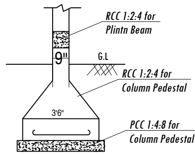
Typical Cross-Section
