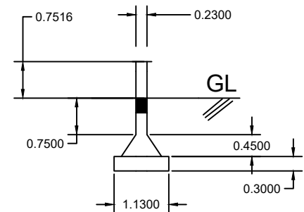
Foundation Details
