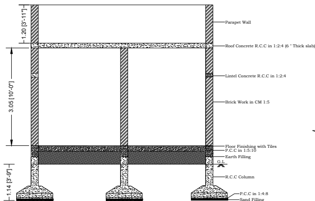
SECTION X-X
