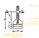
FOUNDATION DETAILS SCALE 1:50
