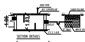
SEPTIC TANK AND DISPERSION TRENCH DETAILS
