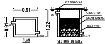
RAINWATER HARVESTING SYSTEM
