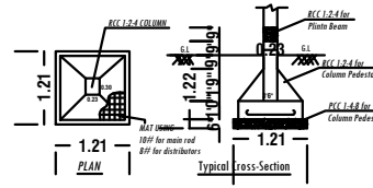
FOOTING DETAILS
