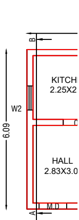
GROUND FLOOR PLAN
