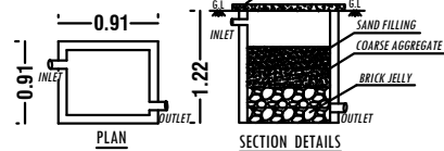
RAINWATER HARVESTING SYSTEM
