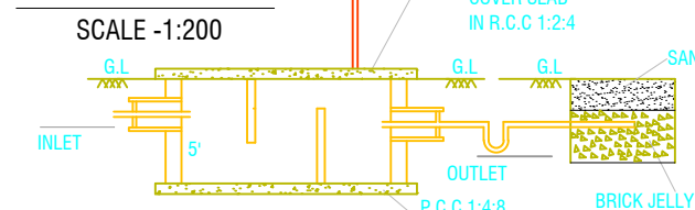
SECTION-AB
