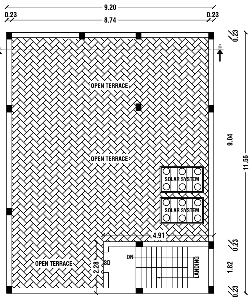
OPEN TERRACE FLOOR PLAN
