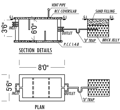
SEPTIC TANK AND DISPERSION TRENCH DETAILS
