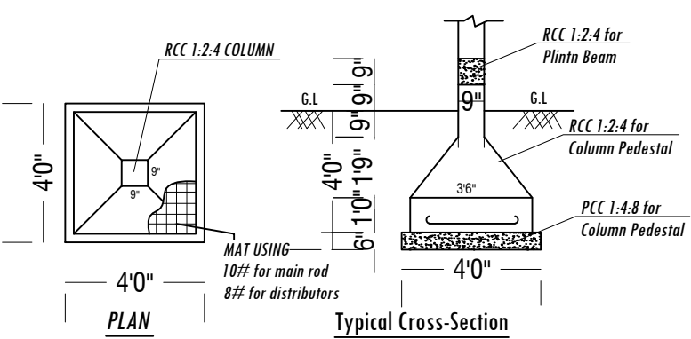
FOOTING DETAILS
