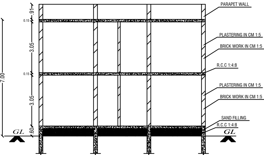
SECTION "US"
