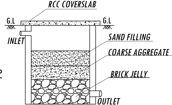
SECTION DETAILS
