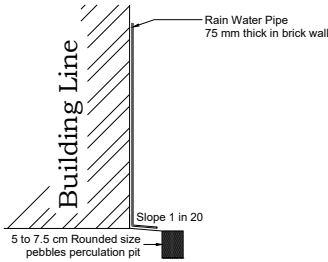
RAINWATER HARVESTING
