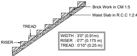
STAIRCASE DETAILS
