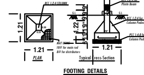
FOOTING DETAILS
