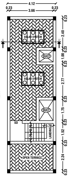
OPEN TERRACE FLOOR PLAN
