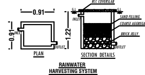
RAINWATER HARVESTING SYSTEM
