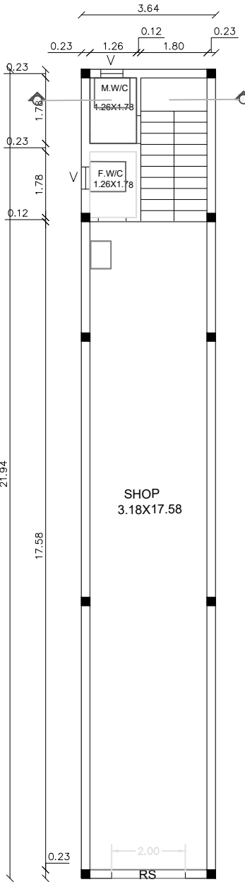
GROUND FLOOR
