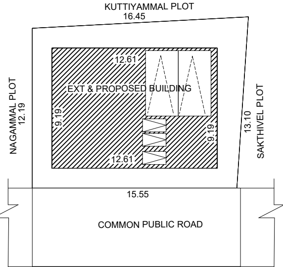
SITE PLAN
