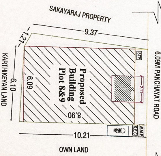
SITE PLAN
