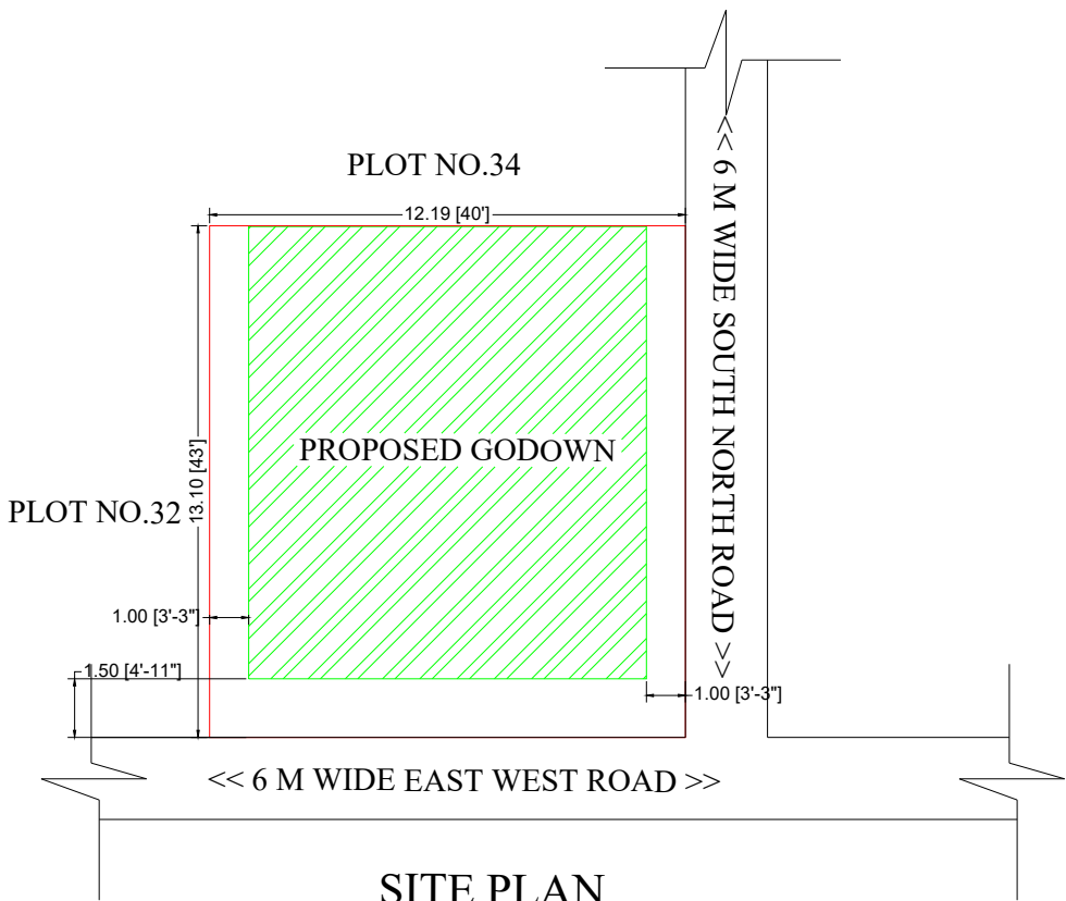
SITE PLAN
