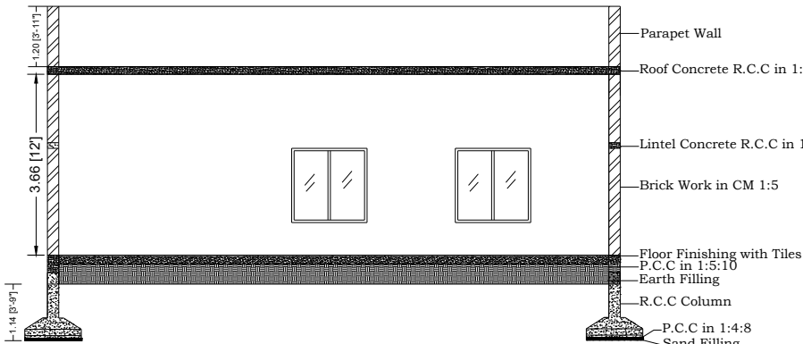
SECTION X-X
