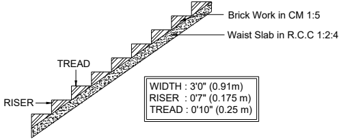
STAIRCASE DETAILS
