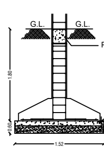
FOUNDATION DETAILS
