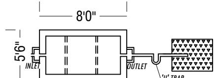
SECTION DETAILS
