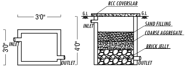
RAINWATER HARVESTING SYSTEM
