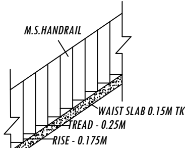
STAIR CASE DETAILS
