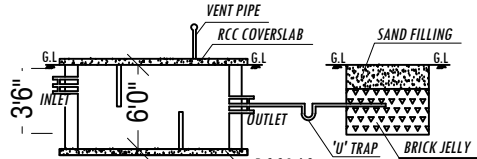
SECTION DETAILS
