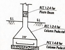
Typical Cross-Section FOOTING DETAILS
