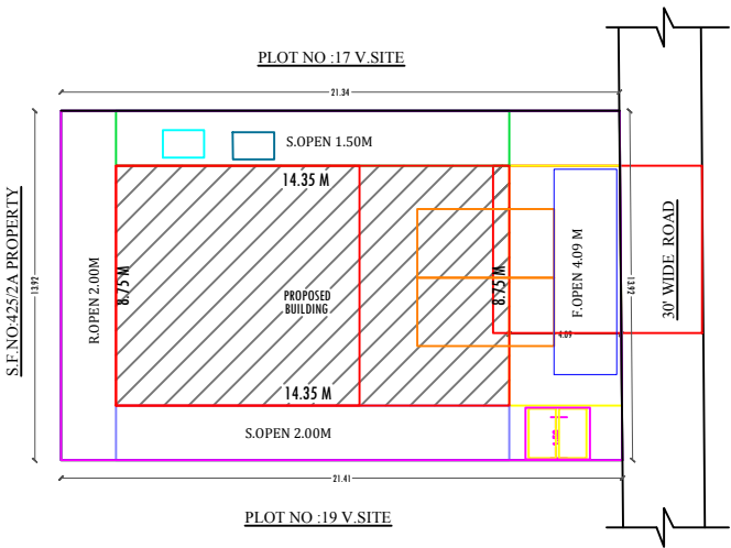
SITE PLAN
