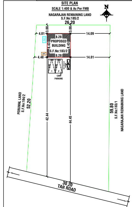
SITE PLAN
