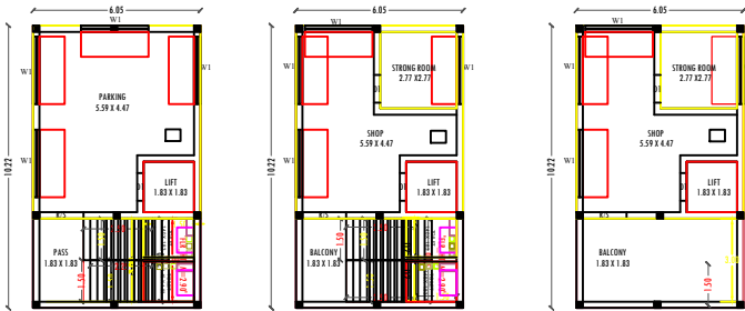
STILT FLOOR PLAN
