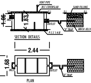
SECTION DETAILS
