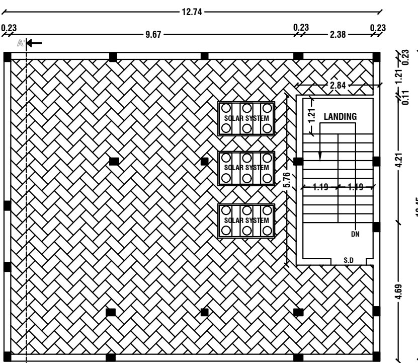
OPEN TERRACE FLOOR PLAN
