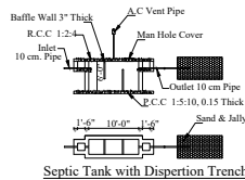
Septic Tank with Dispersion Trench
