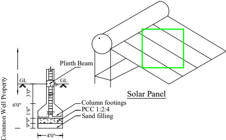
FOUNDATION DETAILS SCALE 1:50
