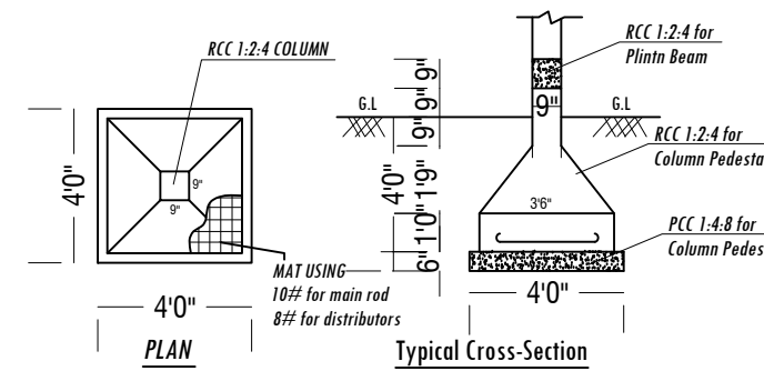
FOOTING DETAILS
