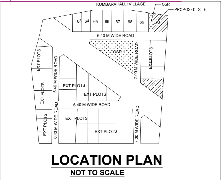
KUMBARAHALLI BOUNDRY 7.92
