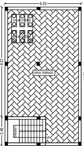
OPEN TERRACE FLOOR PLAN
