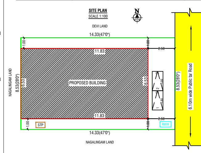
PROPOSED BUILDING
