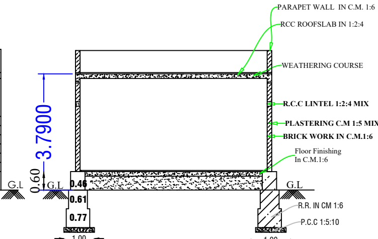
SECTION ON-AA'
