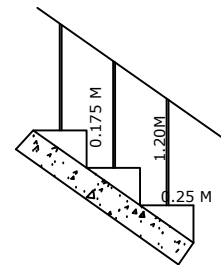
STAIRCASE DETAILS
