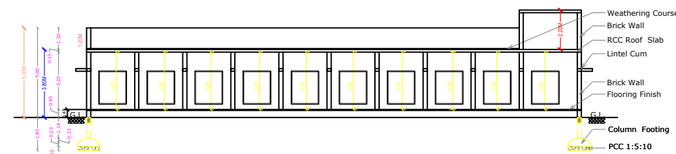
SECTION ON 'AA'
