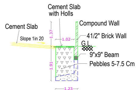
RAIN WATER PERCOLATION BED & COMPOUND WALL
